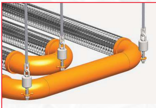
Multiple Breakaway Hangers are ideal for supporting long return bends on nested loops.
