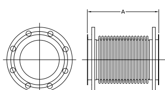
150# FLOATING X 150# C/S FLOATING FLANGES S/S BELOWS
