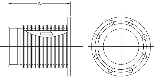
Lip Flange x Flange, w/ Flow Liner
