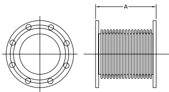
150# FIXED X 150# FIXED C/S FLANGES S/S BELOWS
