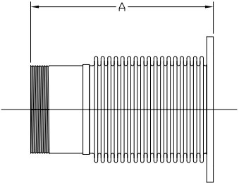
Male NPT x Flange
